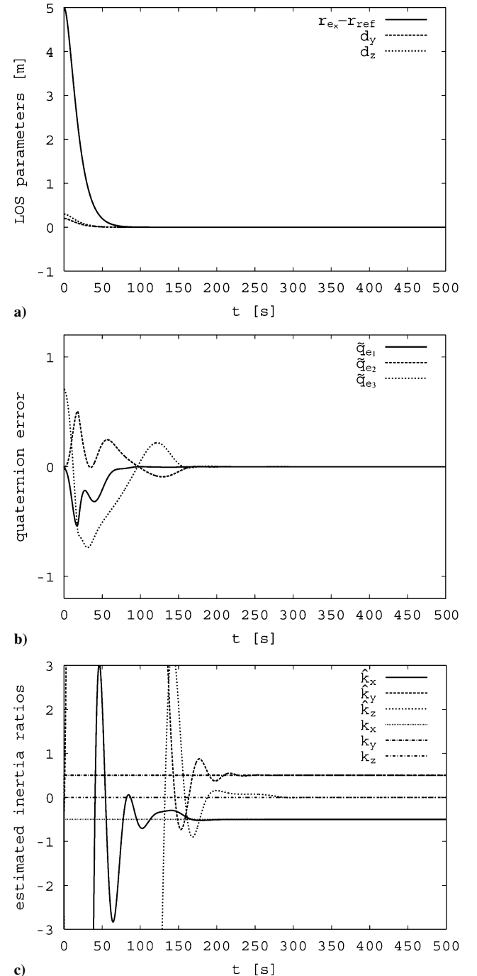
Fig. 1 Time responses of a) LOS parameters, b) quaternion errors, and c) estimated inertia ratios for target satellite.
